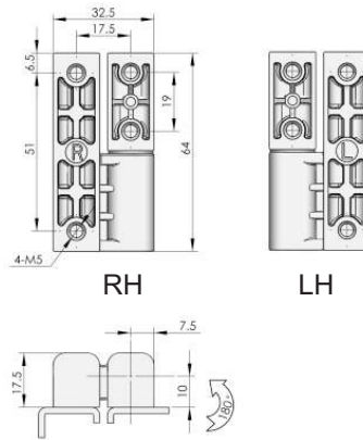
Offset hinge
