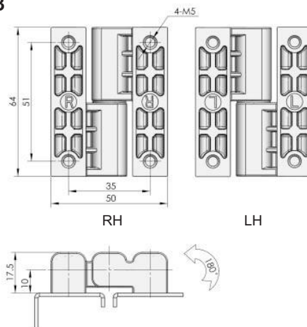
Symmetric hinge
