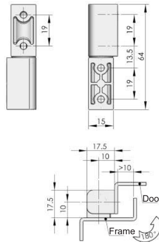
Coaxial hinge
