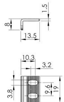
Catcher (Optional)
